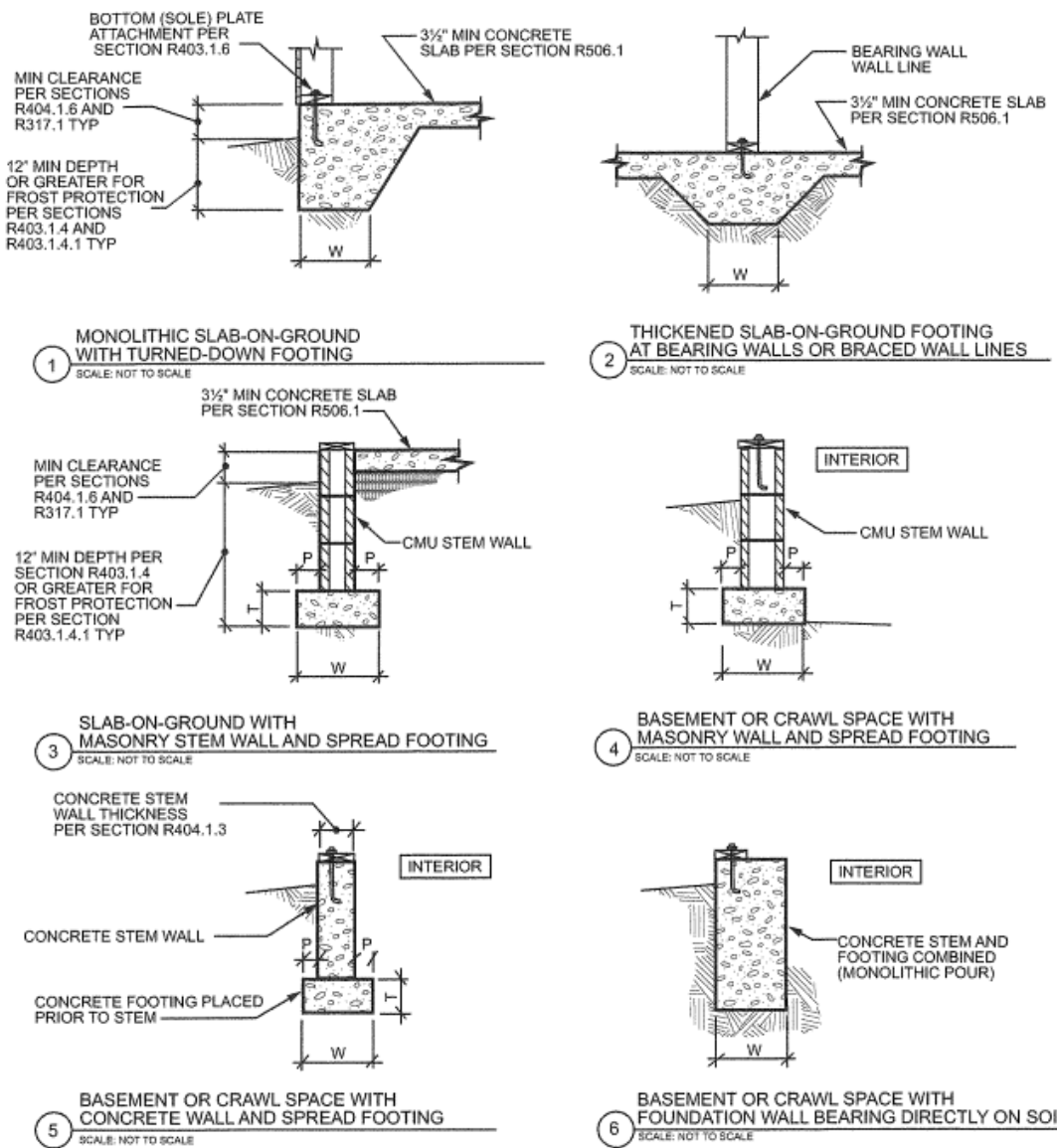
Figure R403.1(1): Plain concrete footings with masonry and concrete stem walls.
